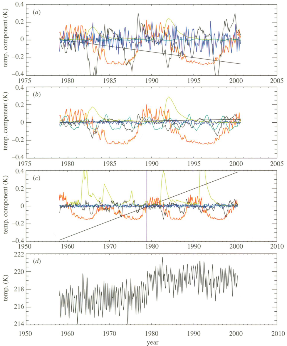
Figure 4. (a) Components of zonal mean temperature anomaly from multiple regression analysis of 1979–2000 data deduced to be due to trend (straight black line), solar variability (red line), volcanic aerosol (green line), QBO (cyan line), NAO (blue line) and ENSO (black line) at (a) 35^{\circ} N, 200 hPa; (b) 35^{\circ} S, 200 hPa. (c) As in (b) using 1958–2000 data. (d) Raw data at 35^{\circ} S, 200 hPa.
