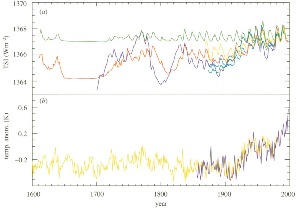
Figure 1. (a) Reconstructions of total solar irradiance from group sunspot numbers, scaled to Nimbus-7 measurements 1979–1993, green line; Lean et al. (1995), red line; Hoyt & Schatten (1993), violet line; Solanki & Fligge (1998), cyan and blue lines; Lockwood & Stamper (1999), yellow line. (b) Reconstructions of surface temperature: global average anomalies relative to 1961–1990 average (Jones et al. 1999), violet line; Northern Hemisphere average (Mann et al. 1998), shifted to match Jones et al. 's record in overlapping period, yellow line. Adapted from figure 2 of Haigh (2000) with permission from the Royal Meteorological Society.
