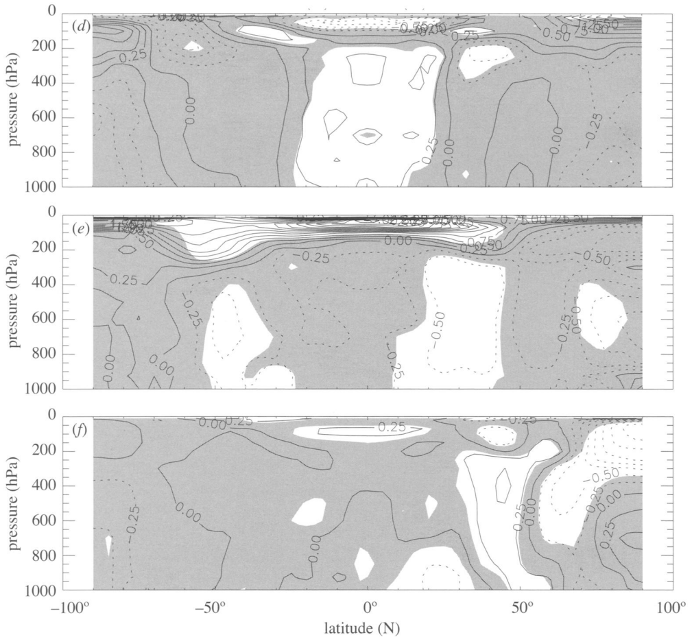
Figure 3. ( Cont. ) Amplitudes of the components of variability in zonal mean temperature due to (d) ENSO (K); (e) volcanoes (K); (f) NAO (K).
