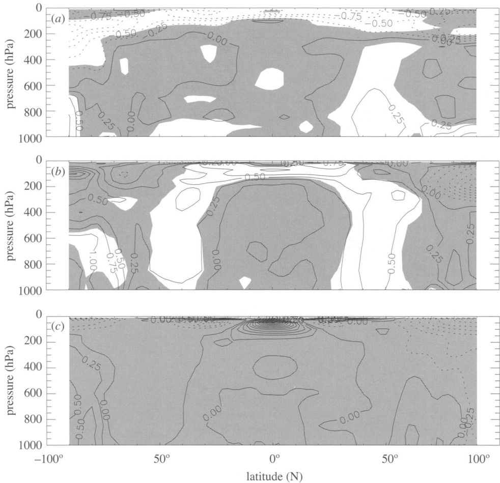
Figure 3. Amplitudes of the components of variability in zonal mean temperature due to (a) trend; (b) solar; (c) QBO. The units are kelvin per decade for the trend, otherwise maximum variation (K) over the data period. Shaded areas are not statistically significant at the 95% level using a student's t-test.
