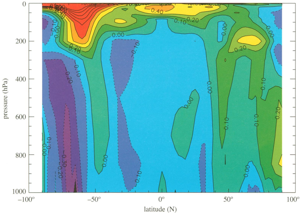
Figure 5. Difference in zonal mean temperature (K) between minimum and maximum of the 11-year solar cycle calculated using an atmospheric GCM in which the spectral composition of the change in irradiance was included in addition to solar-induced changes in ozone (derived off-line using a two-dimensional photochemical/radiative/transport model).
